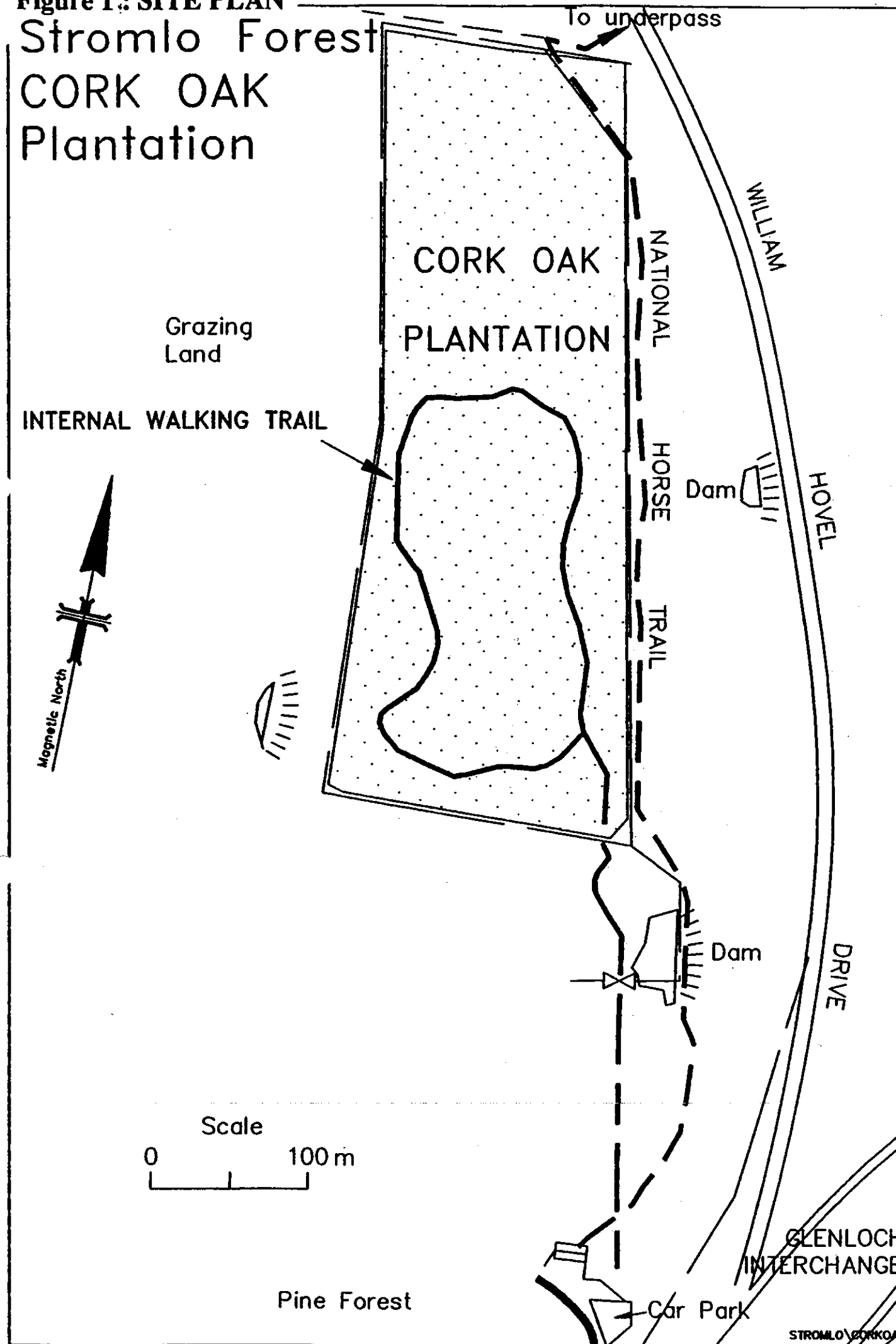
Figure 1: SITE PLAN
